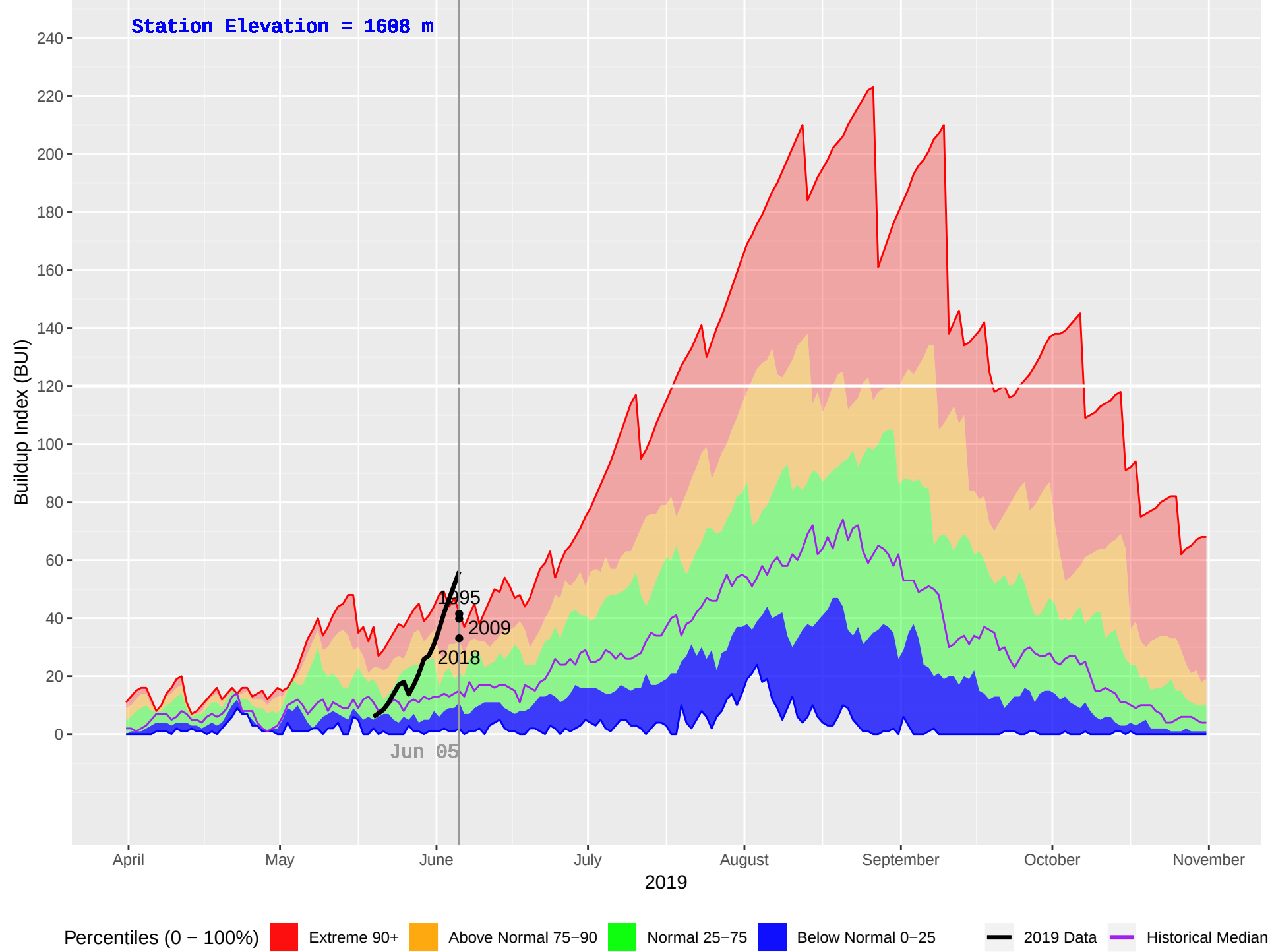
DEWAR CREEK (421) : Historical (1986–2018), Current (2019) Daily Buildup Index (BUI)
