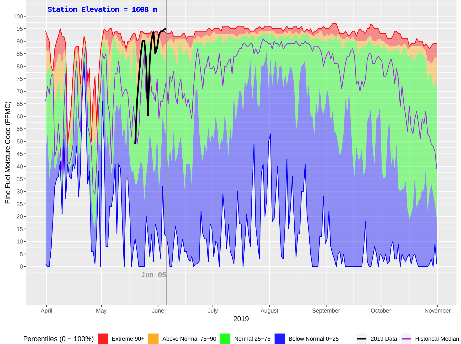
DEWAR CREEK (421) : Historical (1986–2018) and Current (2019) Daily Fine Fuel Moisture Code (FFMC)
