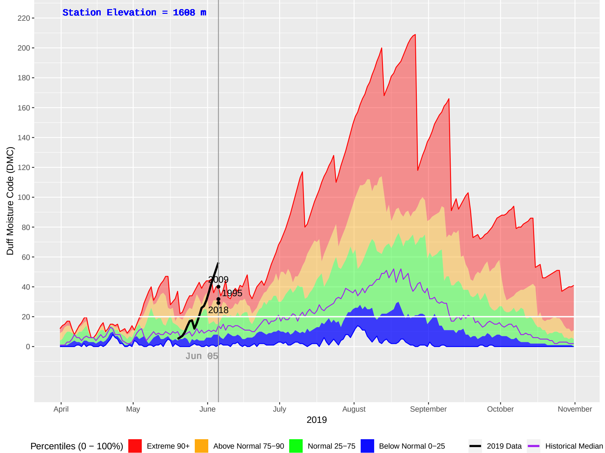
DEWAR CREEK (421) : Historical (1986–2018), Current (2019) Daily Duff Moisture Code (DMC)
