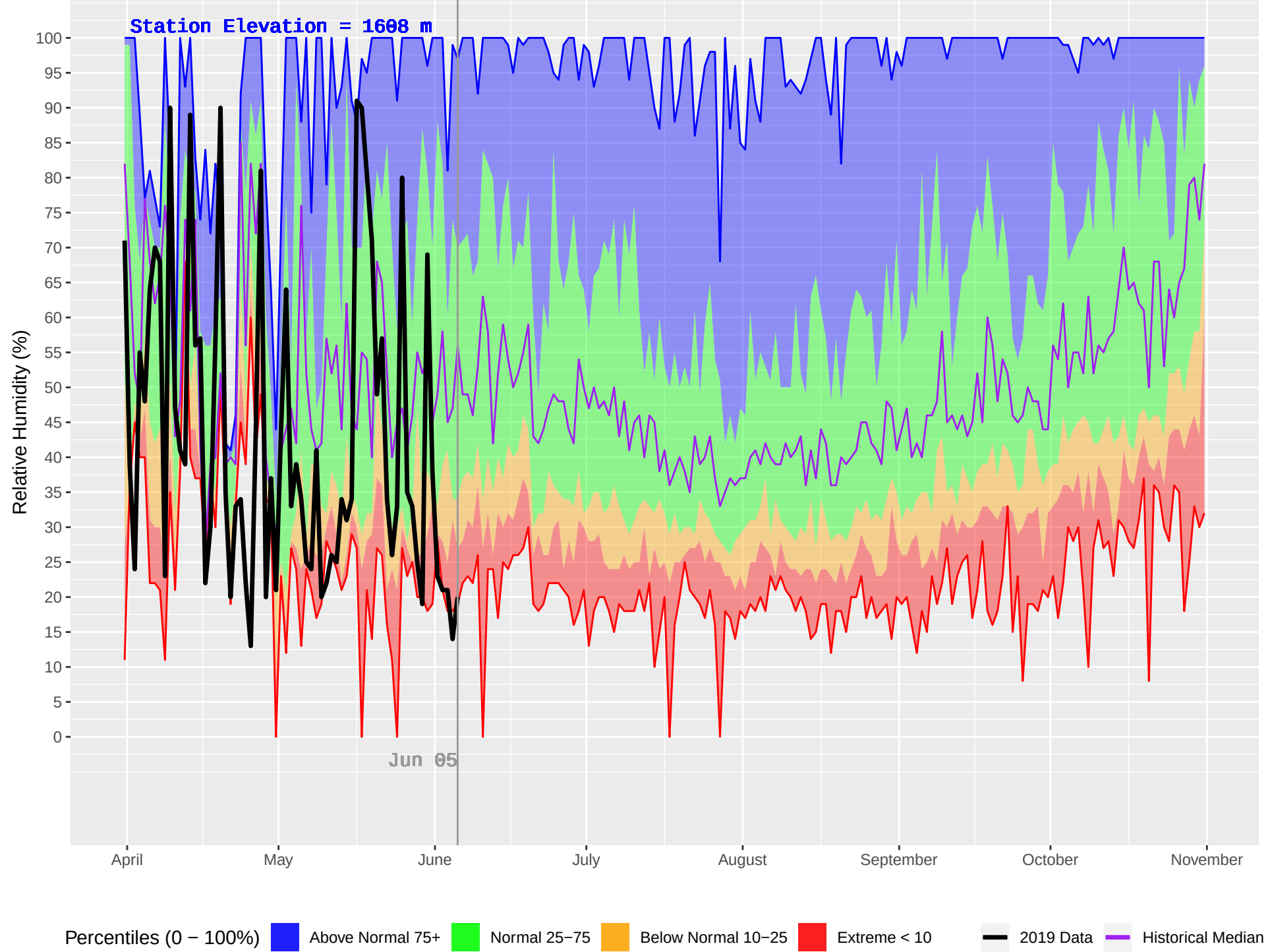
DEWAR CREEK (421) : Historical (1986–2018) and Current (2019) Daily Relative Humidity
