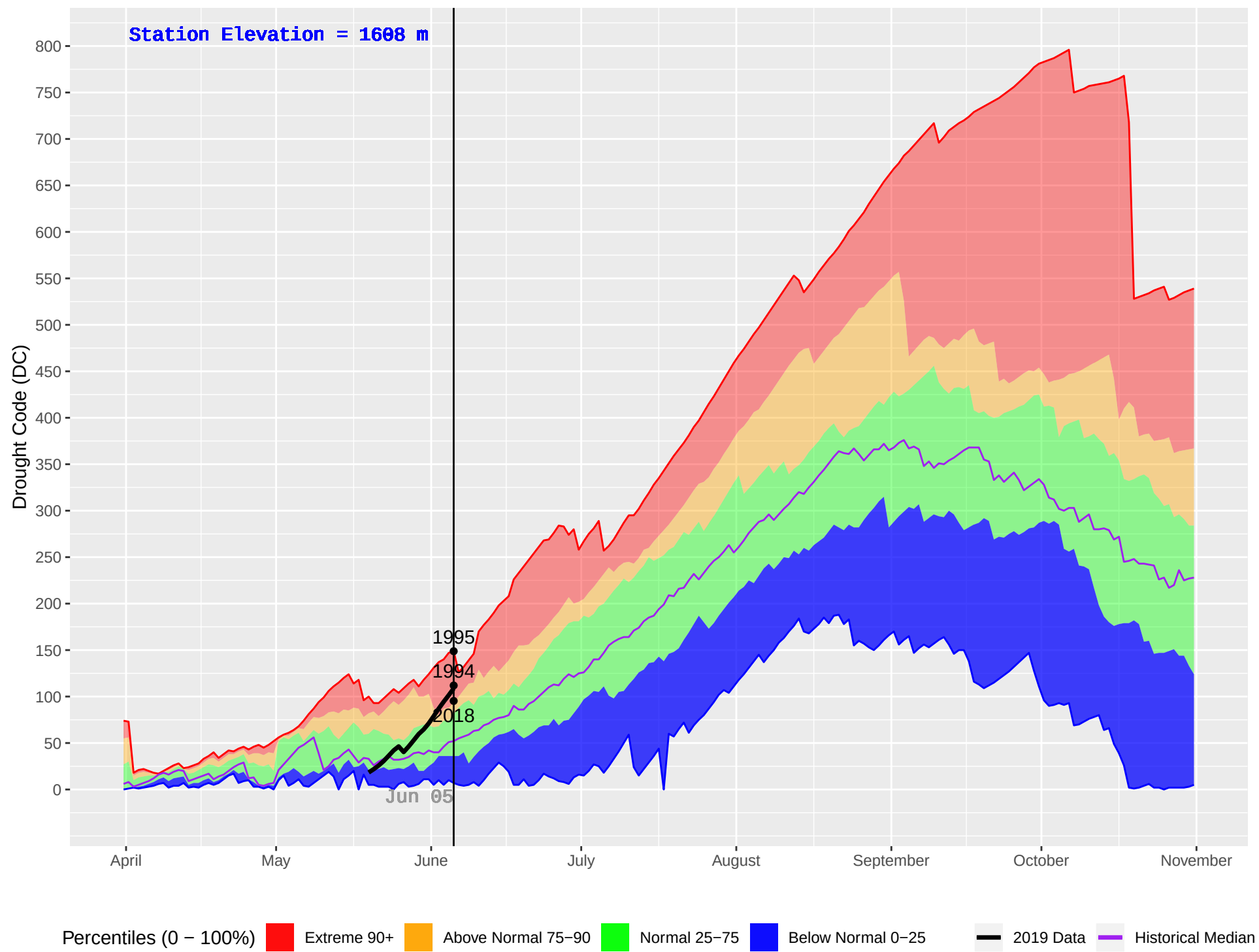
DEWAR CREEK (421) : Historical (1986–2018) and Current (2019) Daily Drought Code (DC)
